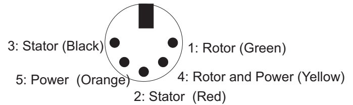
5 Pin DIN Female Connector
